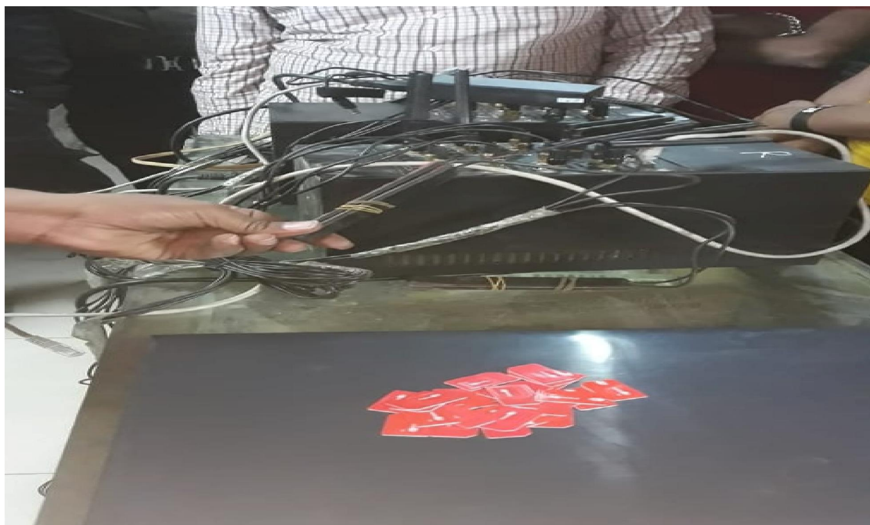
Pictures of the confiscated Equipment & apparatus: (SIMBOX ,GSM Antenna, Wireless Router of QUBEE & TP-Link)
